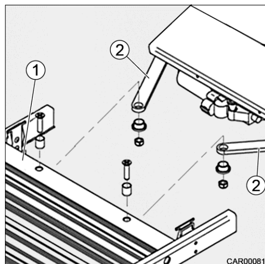
Afb. 10 Noodontgrendeling
