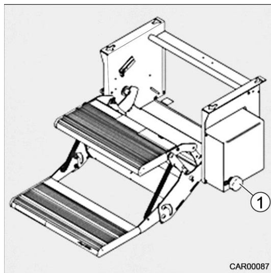
Afb. 15 Noodontgrendeling
